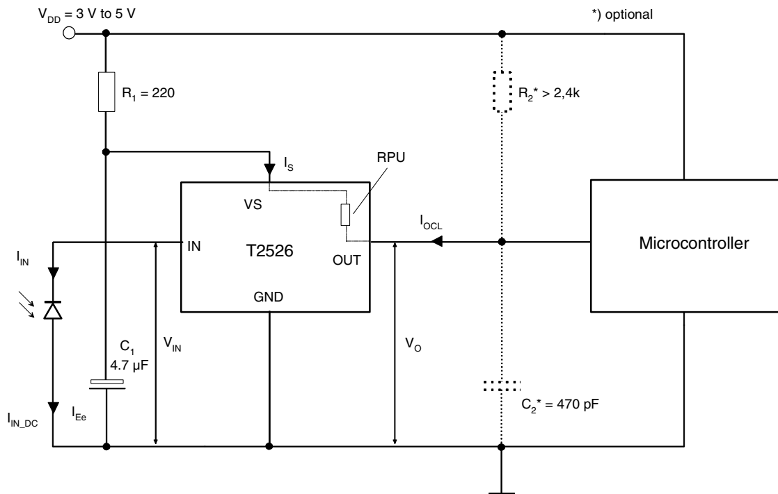
Figure 12. Application Circuit
